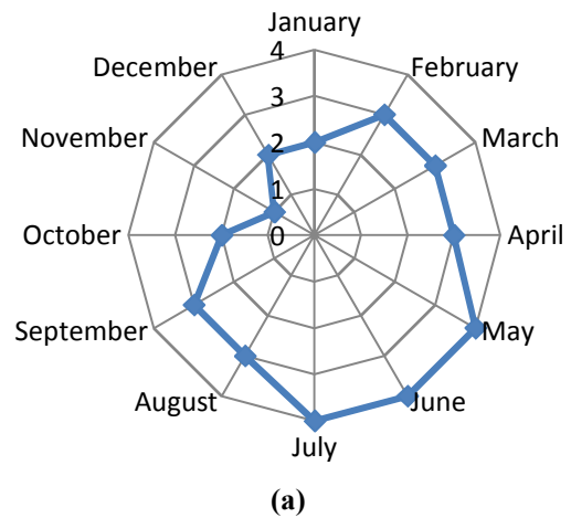
Fig. 4. Dew point (°C) in district Kurukshetra, Haryana (India) from January, 2016 to December, 2016.
