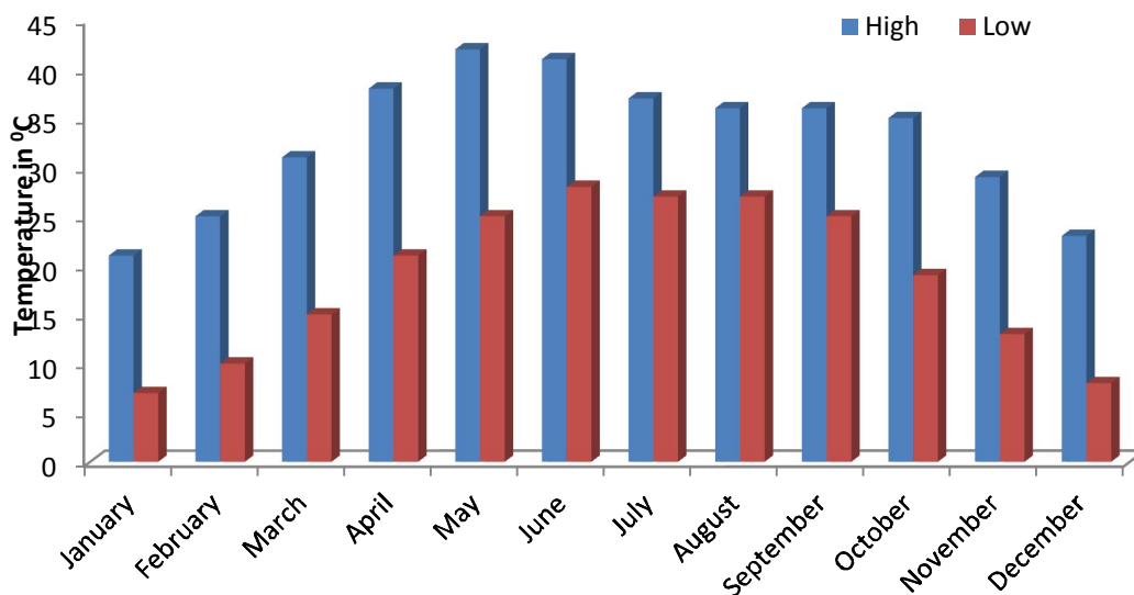
Fig. 1. Temperature variation (high and low) in district Kurukshetra, Haryana (India) from January, 2016 to December, 2016.
