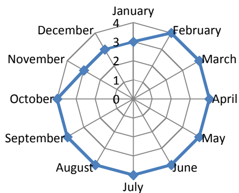
Fig. 5. (a) Wind (Km/h), (b) pressure (mbar) and (c) visibility/Km in district Kurukshetra, Haryana (India) from January, 2016 to December, 2016.
