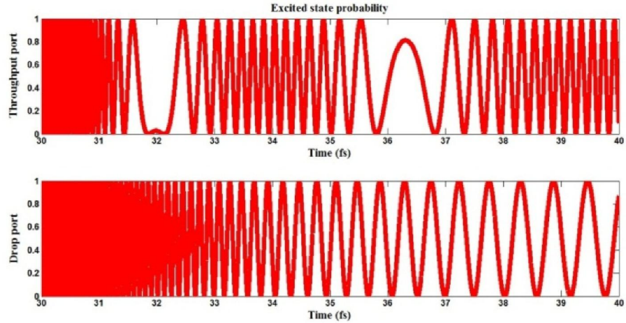
Figure 4: Rabi oscillation signals at Throughput (top) and Drop (bottom) ports
