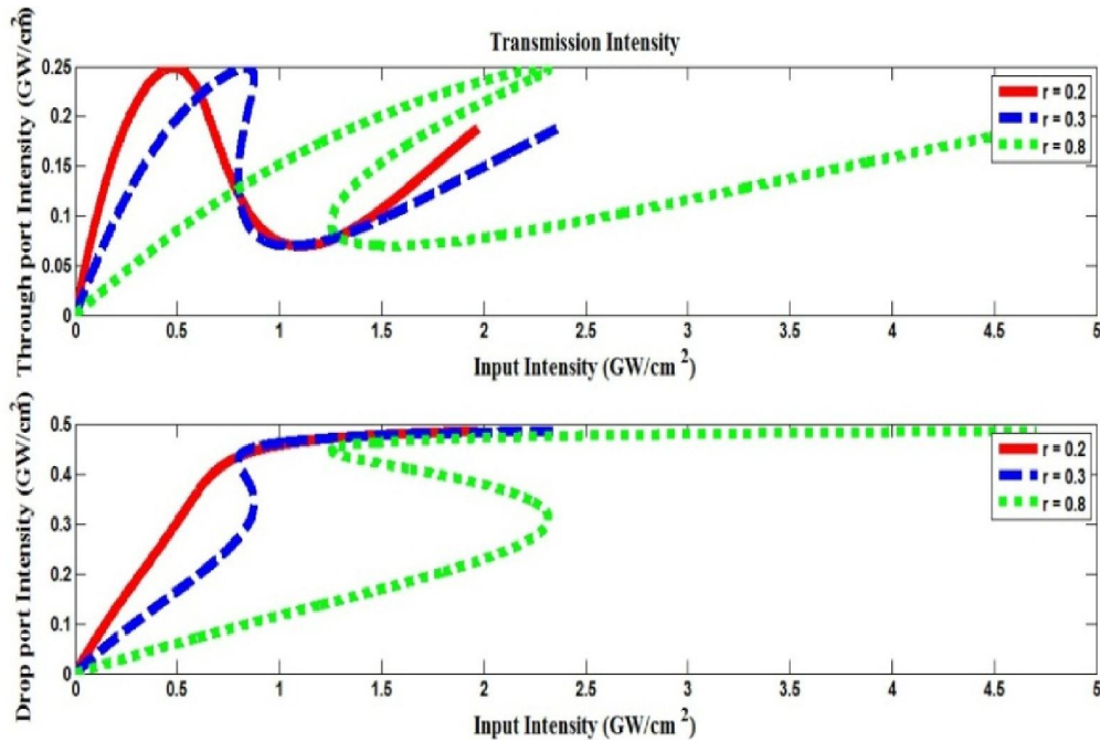
Figure 3: Plot of photon nonlinearity behavior, i.e. bistability with different coupling coefficients ( r )
