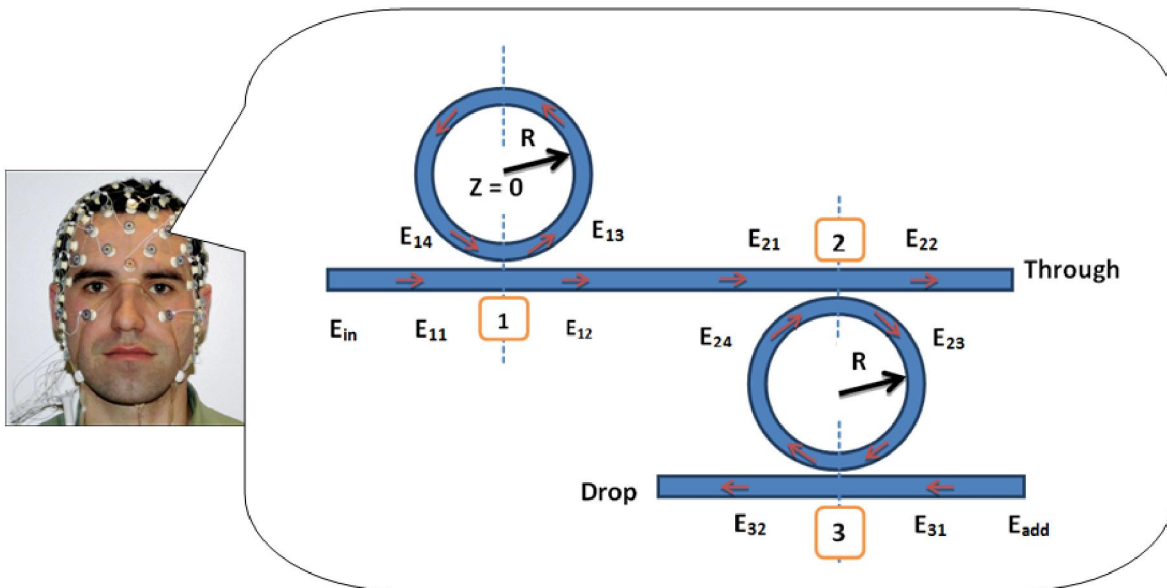
Figure 1: The proposed Rabi oscillation system, where E_i : optical fields, R : ring radius, Drop: drop port, E_{dd} : add port, Through: throughput port; 1, 2, 3: coupling coefficients ( r ) at points 1, 2 and 3 (Pantian & Yupapin, 2013)
