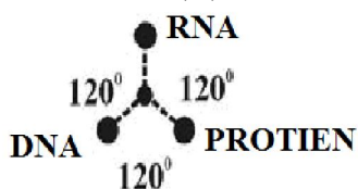
(Particle Oscillation)
