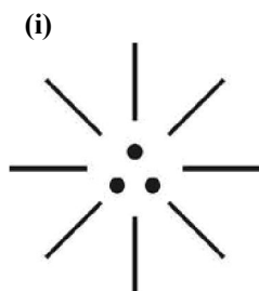
(NEUTRINO CELL)
