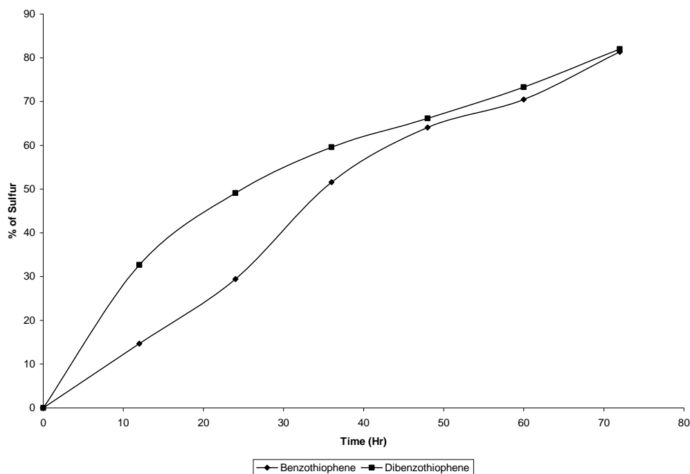
Figure 5: The Percentage Desulfurization -Time Profile of benzothiophene and dibenzothiophene Biodesulfurization by Desulfobacterium anilini
